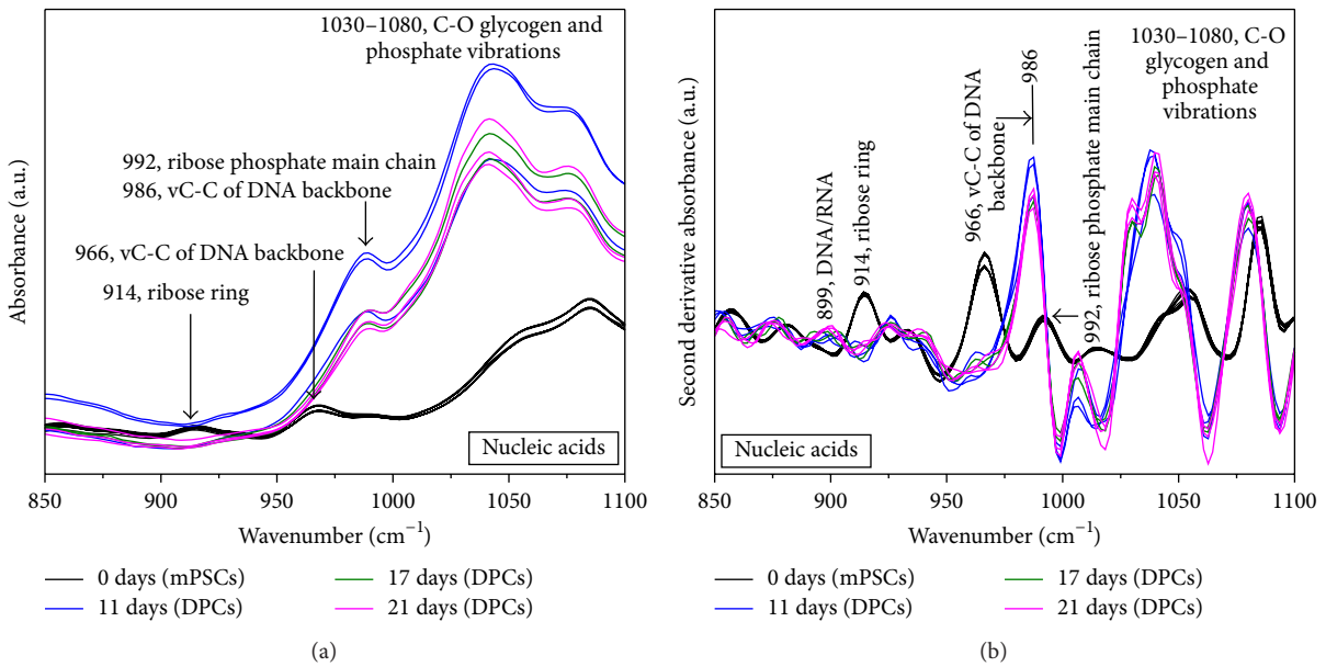
FIGURE 5: FTIR spectra of mouse pluripotent stem cells (mPSCs) and Differentiated Pancreatic Cells (DPCs) at different maturation stages (11, 17, and 21 days) depicted in the nucleic acids region ( N = 3 ). (a) Raw spectra. (b) Second derivative of absorbance.
