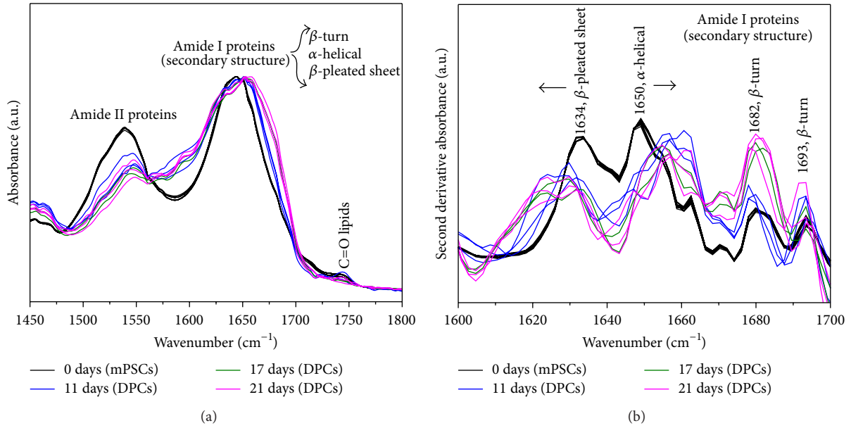
FIGURE 4: FTIR spectra of mouse pluripotent stem cells (mPSCs) and Differentiated Pancreatic Cells (DPCs) at different maturation stages (11, 17, and 21 days) depicted in the amide I and amide II region ( N = 3 ). (a) Raw spectra. (b) Second derivative of absorbance.
